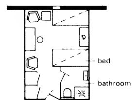
19 Twin cabin with shower/toilet
